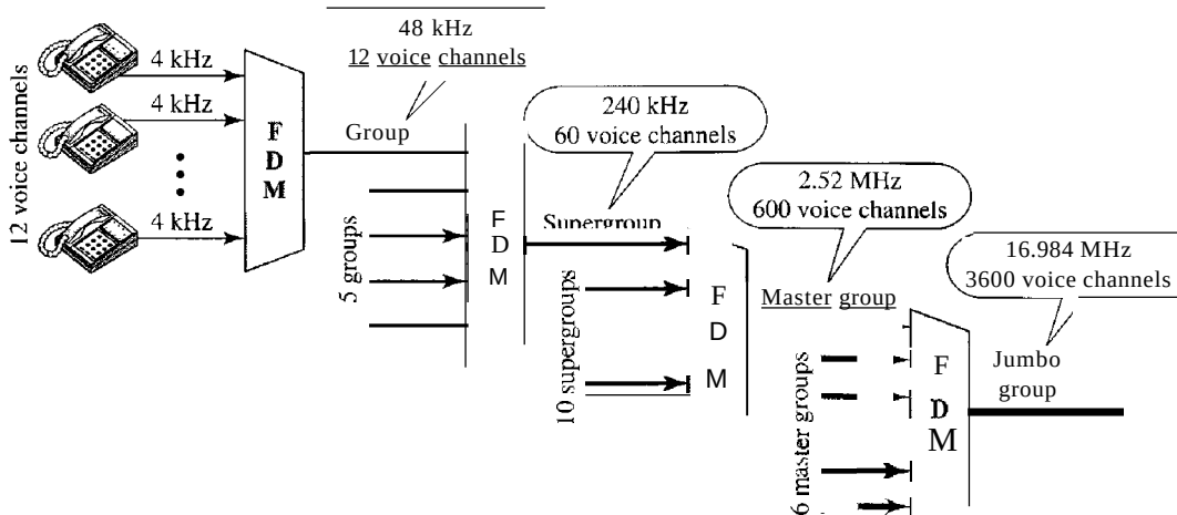
Figure 6.9 Analog hierarchy
