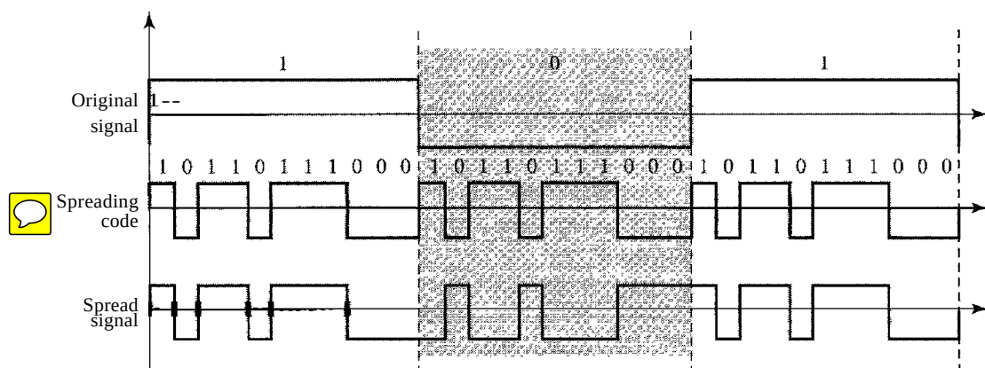
Figure 6.33 DSSS example
